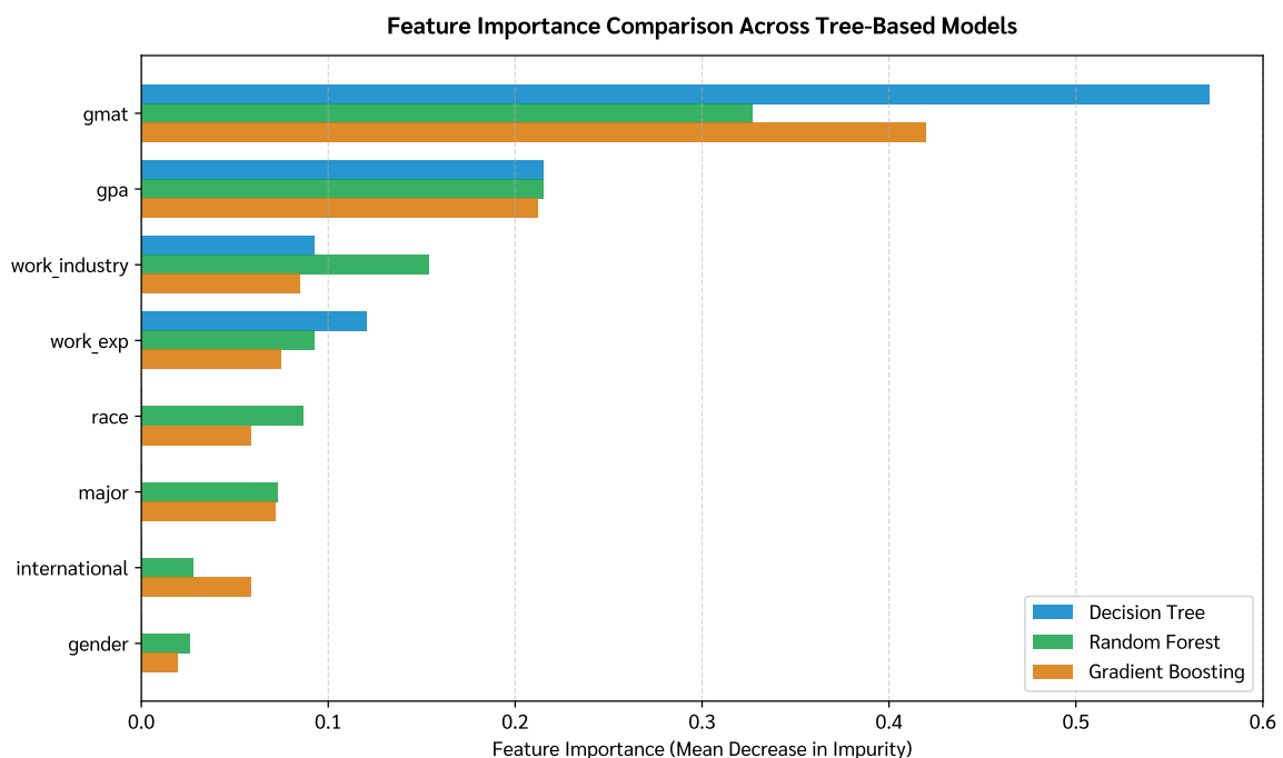
Figure 3 (Feature Importance Comparison): Horizontal bar chart comparing relative feature importances derived from Mean Decrease in Impurity. GMAT score, GPA, Work Experience, and Work Industry emerge as the dominant predictors across all three architectures, while demographic indicators (gender, race, international) exhibit lower direct influence.
